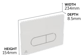
Oleas M1 Mechanical Dual Flushplate
