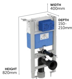
820mm Wall Hung WC Frame
