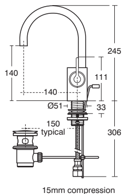
15mm compression
