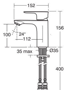
15mm compression
