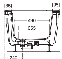
Section B - B
