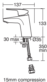
15mm compression
