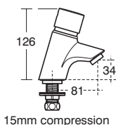
15mm compression
