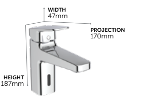
Single Lever Sensor Hybrid Basin Mixer
