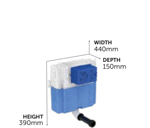
150 Depth Concealed Cistern, Furniture Height
