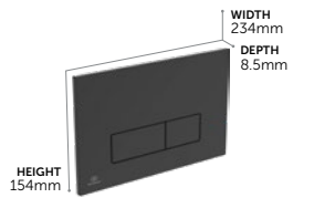
Oleas M2 Mechanical Dual Flushplate
