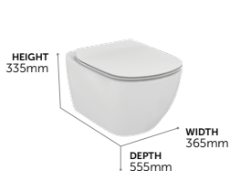
AquaBlade® Wall Mounted Toilet
