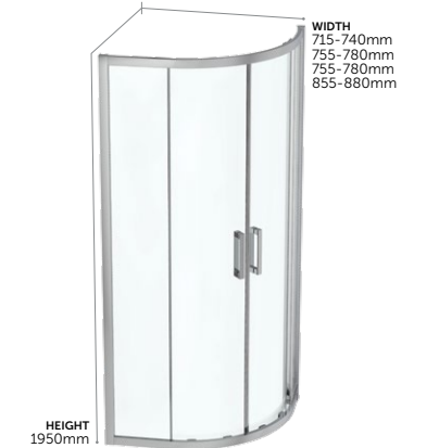
Offset Quadrant Enclosures
