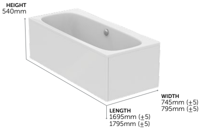
Double Ended Bath
