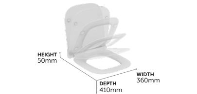
Compact Slim Toilet Seats and Covers
