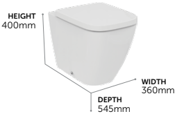
Back to Wall Toilet with RimLS+
