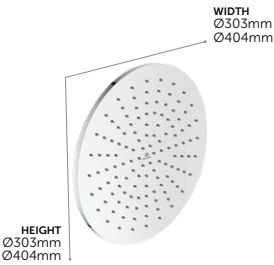
Round Ø300mm/400mm Rainshowers
