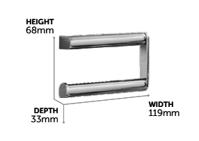
Toilet Roll Holder N1381AA £73
