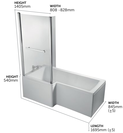
Space Square Shower Bath 170 cm
