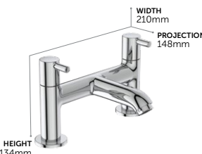
Dual Control Bath Filler
