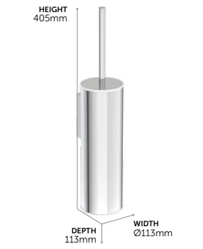
Toilet Brush & Holder N1396AA £121
