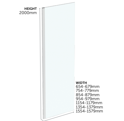
i.life Wet Room Panel
