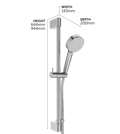
Round Ø100mm 2 Function Shower Set
