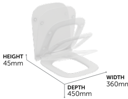
Slim Toilet Seats and Covers
