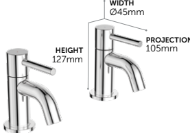
Bath Pillar Taps
