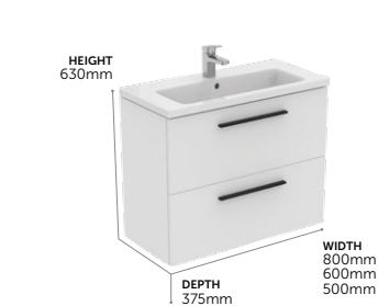
Compact Basin Unit, 2 Drawers
