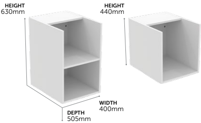
Open Side Unit, for Worktops, 40 cm
